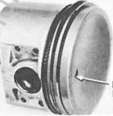
PISTON STABILISING BANDS
