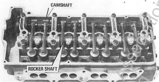
CAMSHAFT AND ROCKER SHAFT BEARING CAPS
