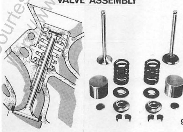
VALVE ASSEMBLY
