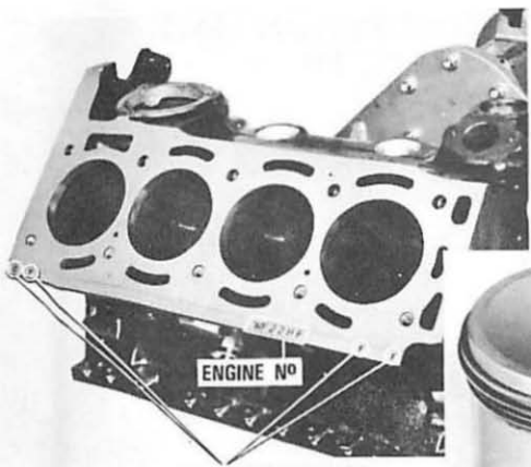
CYLINDER BORE GRADE LETTERS
