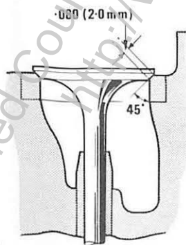
CORRECTLY SEATED VALVE
