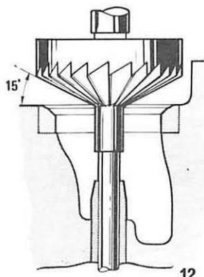
SEAT WIDTH REDUCING CUTTER
